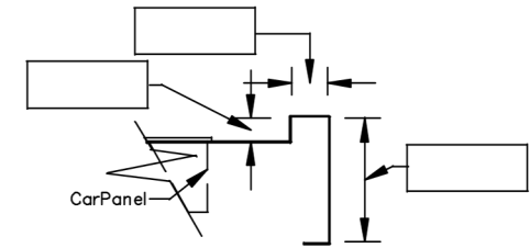
Projected Jamb Detail
