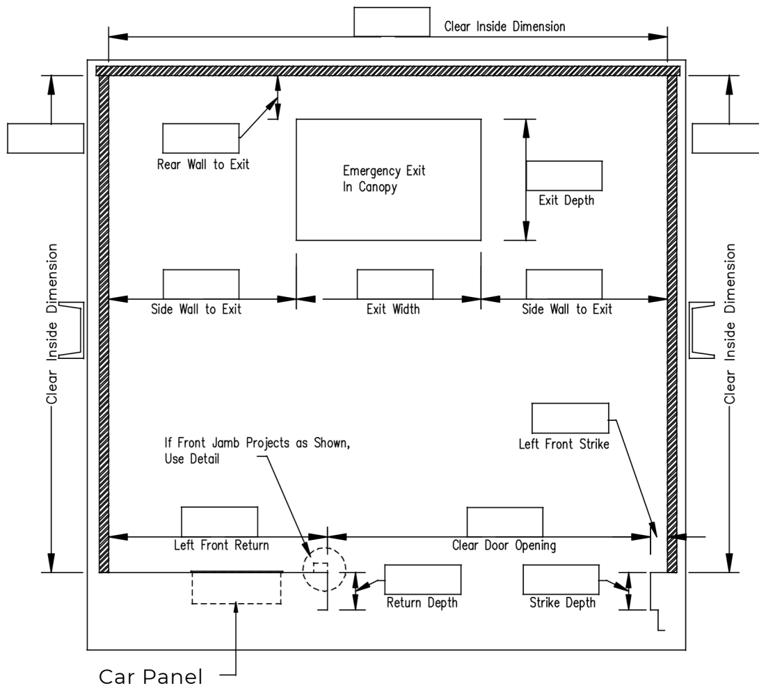
PLAN VIEW Right Hand Opening
