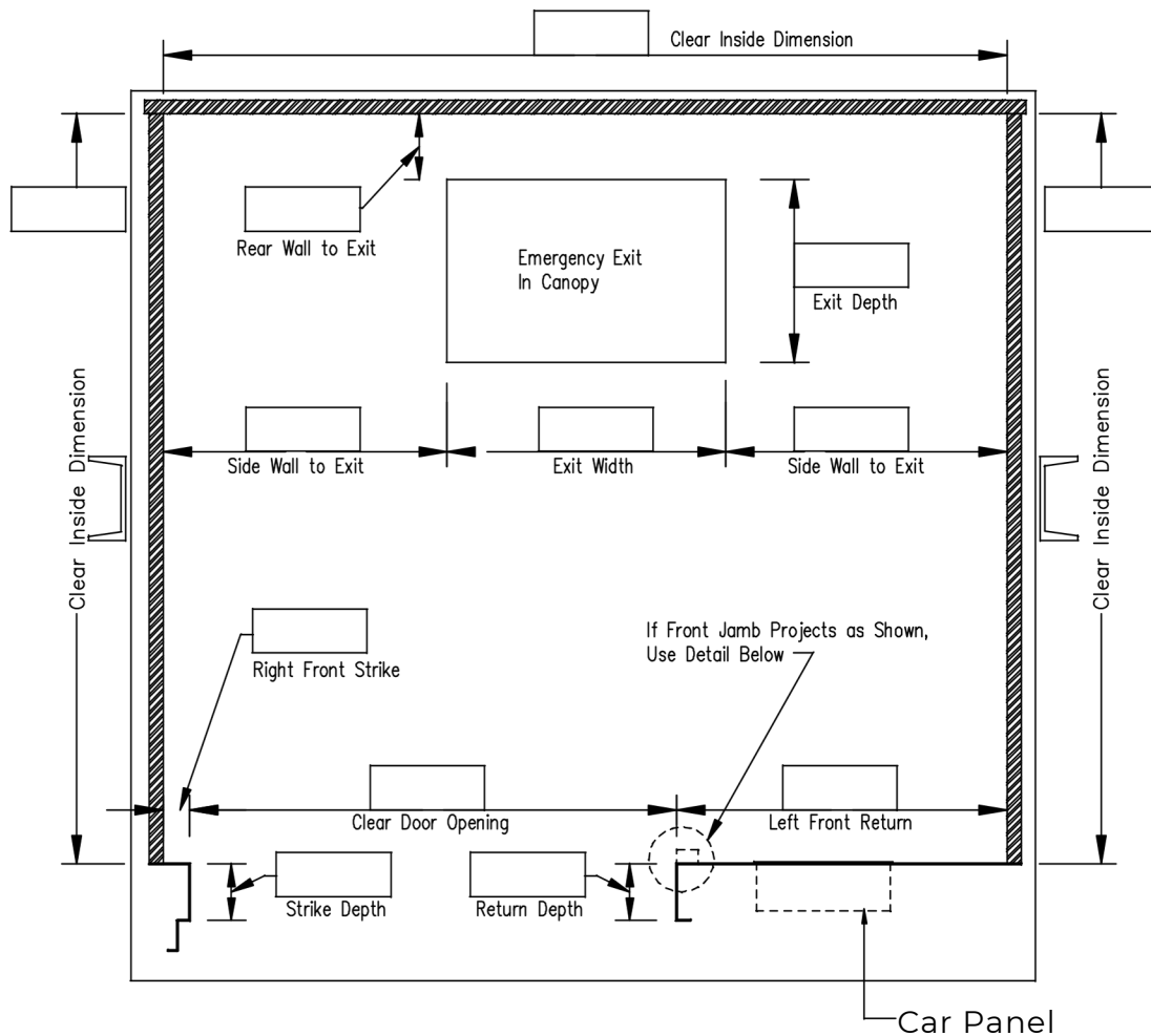
PLAN VIEW Left Hand Opening
