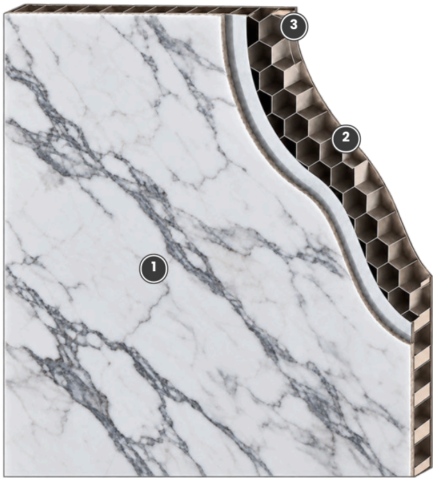
CUTAWAY – 1/4" NATURAL STONE VENEER ON ALUMINUM HONEYCOMB
