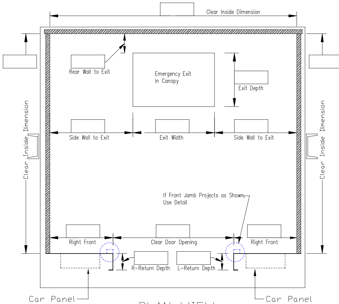
PLAN VIEW Single Speed Center Opening
