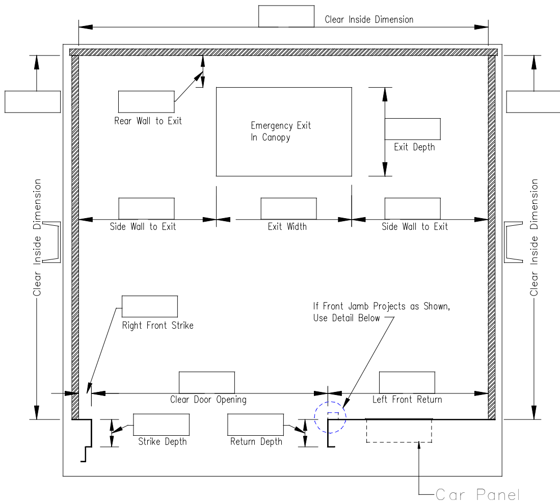
PLAN VIEW Single Speed Side Slide Left Hand Opening
