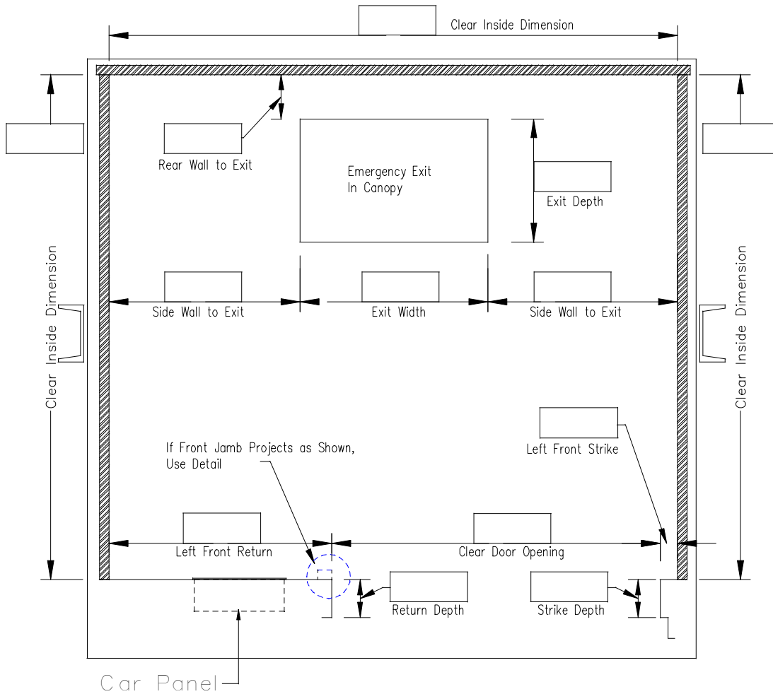
PLAN VIEW Single Speed Side Slide Right Hand Opening
